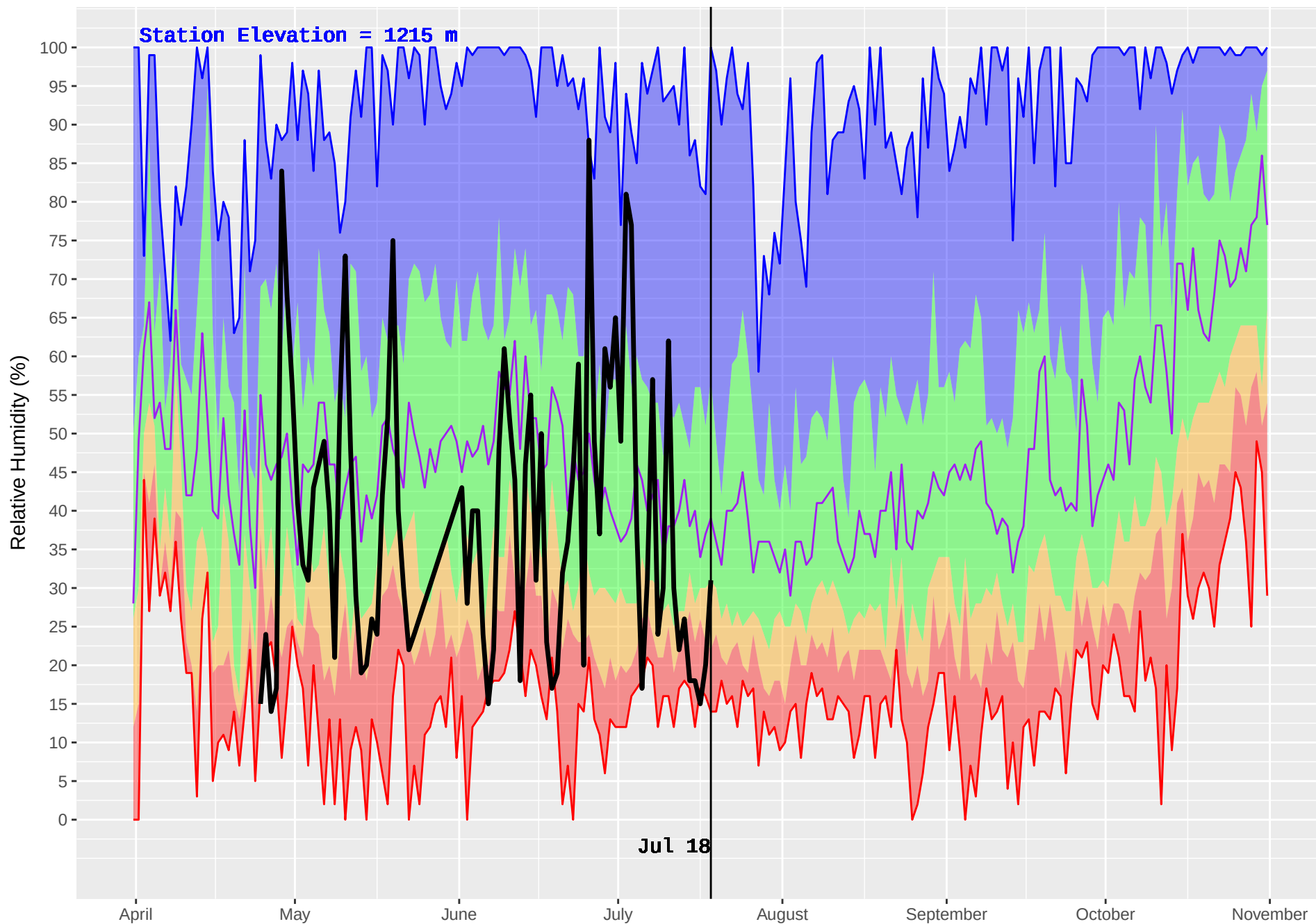
ALLISON PASS (317) : Historical (1987–2016) and Current (2018) Daily Relative Humidity
