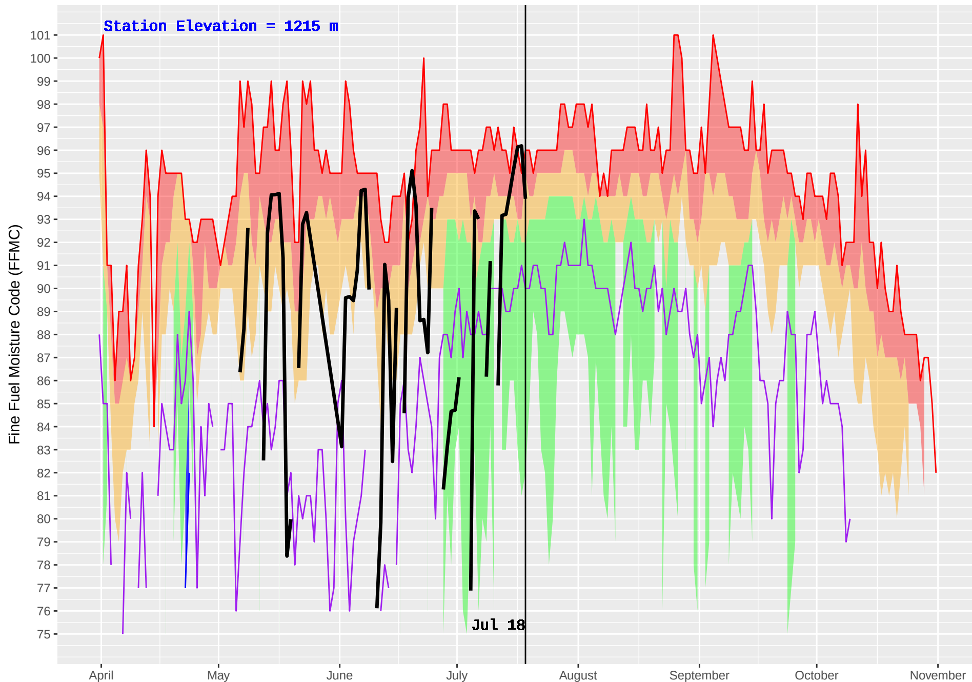
ALLISON PASS (317) : Historical (1987–2016) and Current (2018) Daily Fine Fuel Moisture Code (FFMC)
